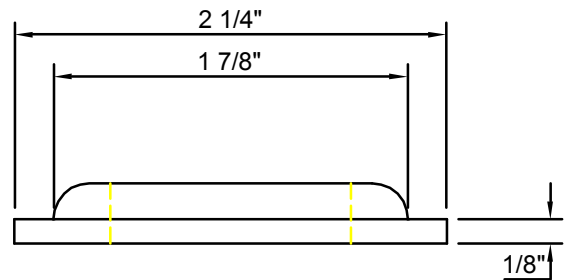
Washer - Side View
