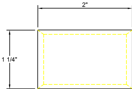
Spacer - Side View
