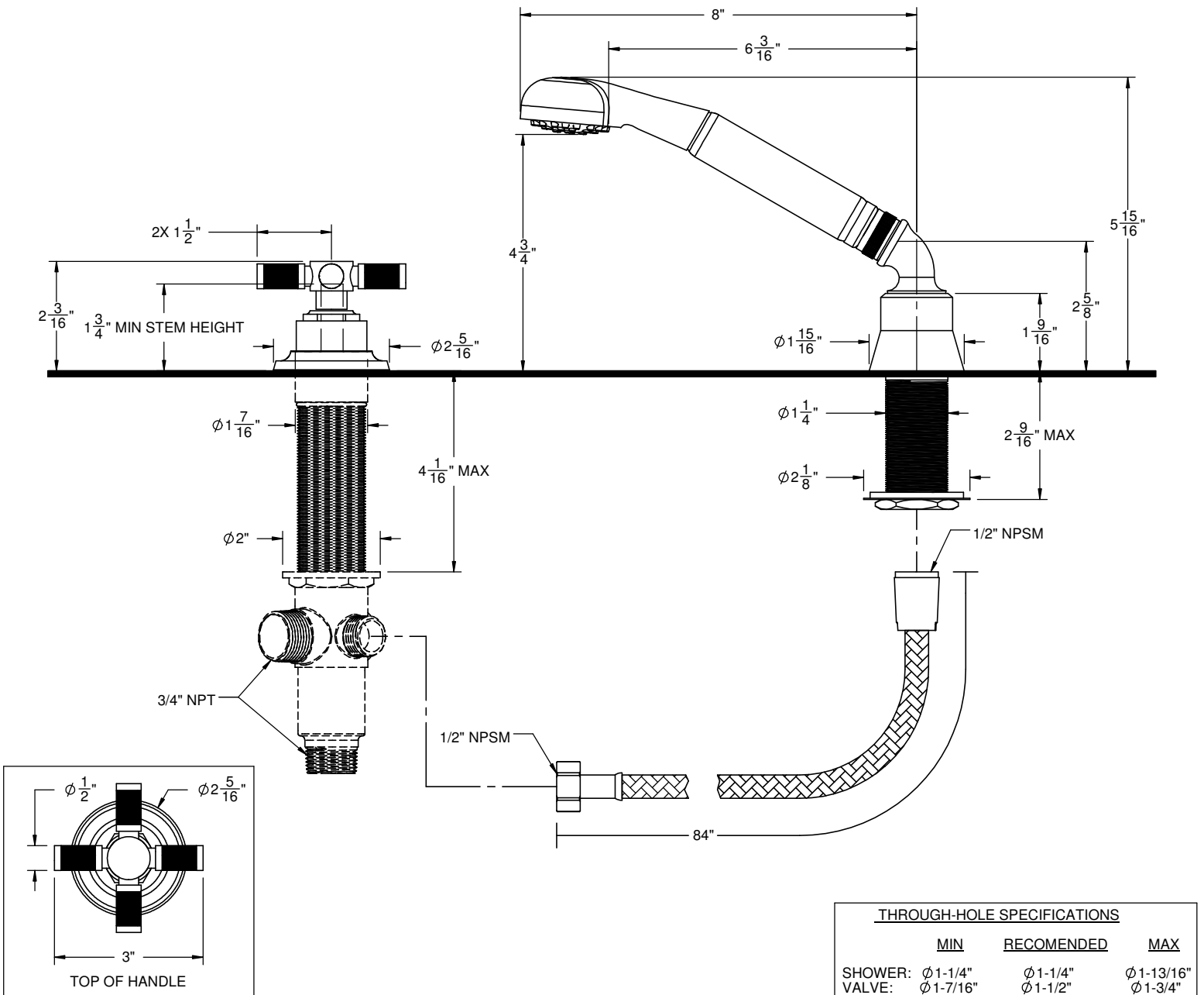
(TO-30X.15S.20 SHOWN)
